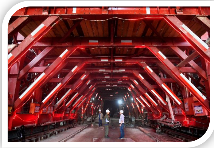
Beijing – Zhangjiakou High Speed Rail under construction
